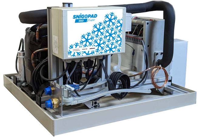
Water cooling
