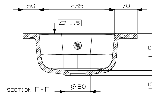
SECTION F-F
