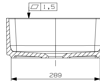
SECTION D-D SCALE 1:5
