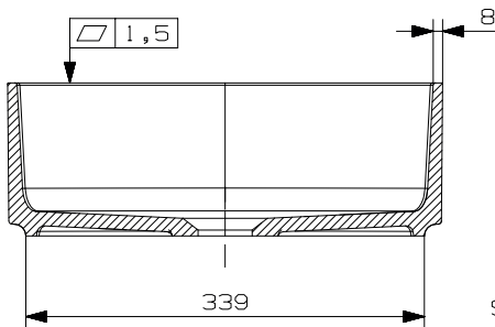
SECTION D-D SCALE 1:5
