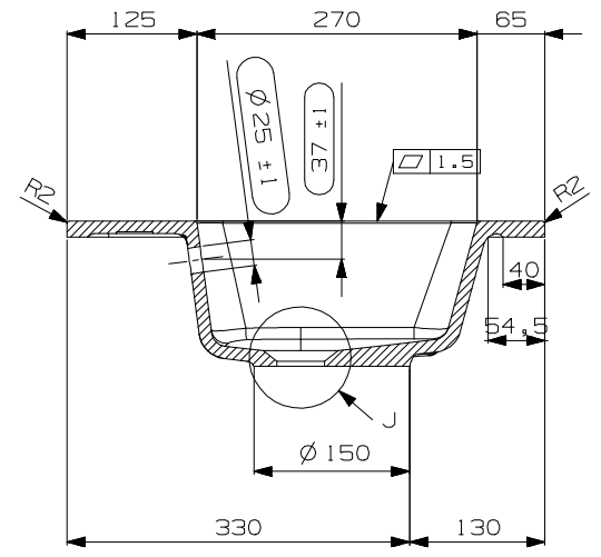
SECTION G-G SCALE 35:200
