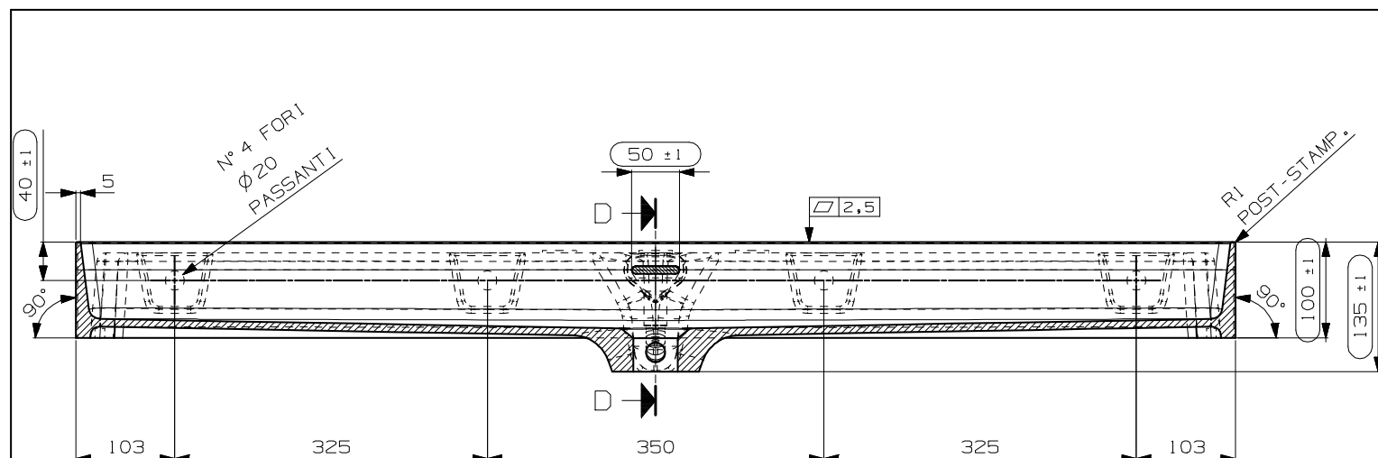
SECTION C-C SCALE 1:5
