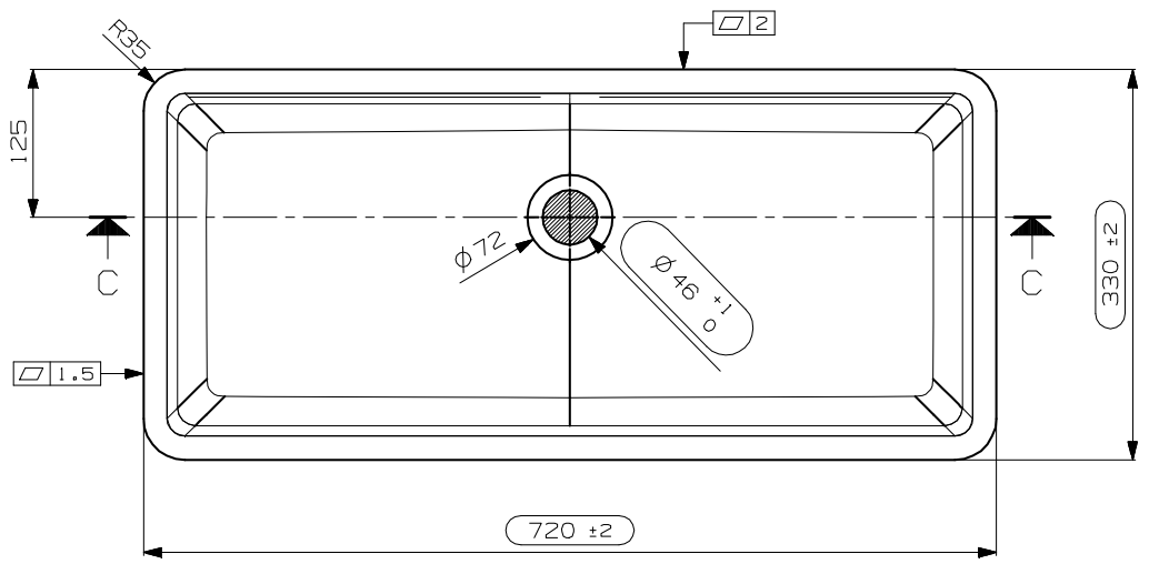
SCALE 1:5
