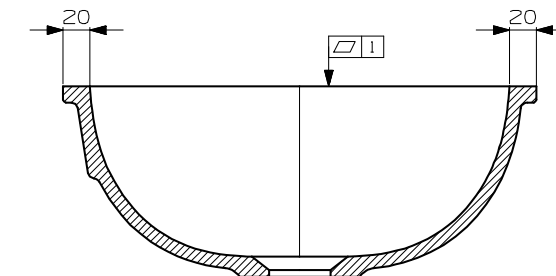
SECTION B-B SCALE 1:4
