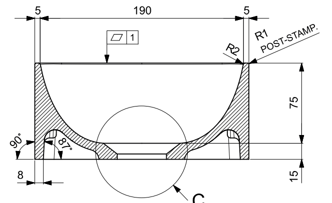
SECTION B-B SCALE 2:5
