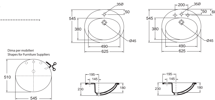
Lavabo incasso JOLLY max monoforo. JOLLY MAX inset one-hole washbasin
